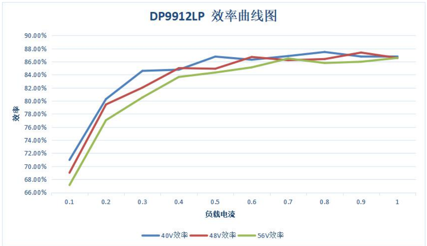
DP9912LP Test efficiency graph
